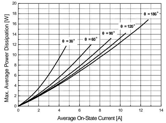
Fig 8. Power Dissipation
